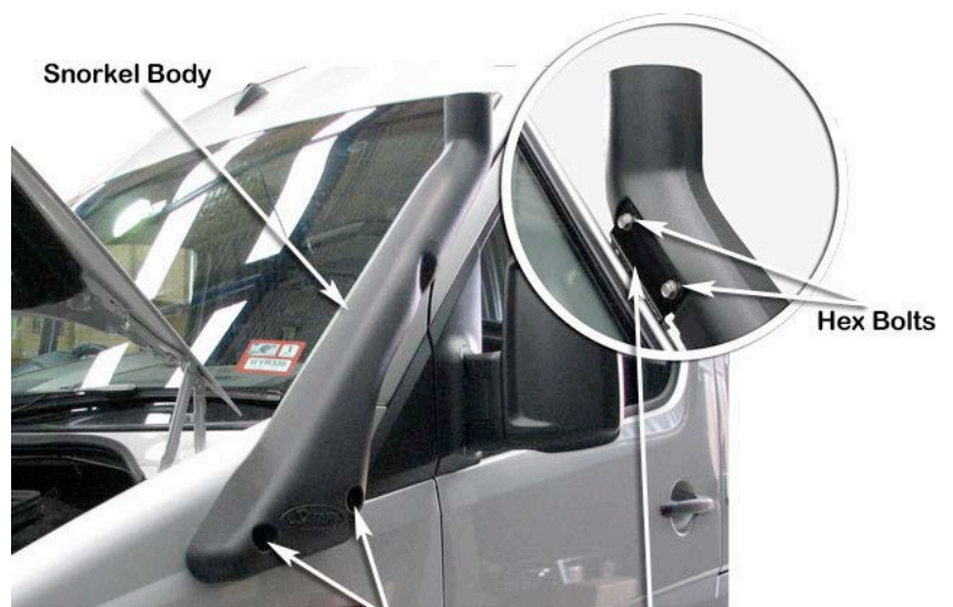
6mm Body Washers & Socket Head Bolts Upper Mounting Bracket
